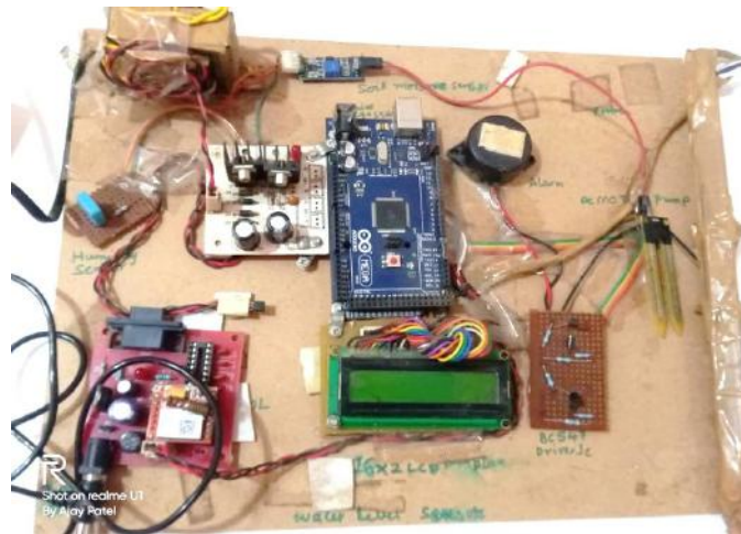
Figure 2: System- Design Implementation
