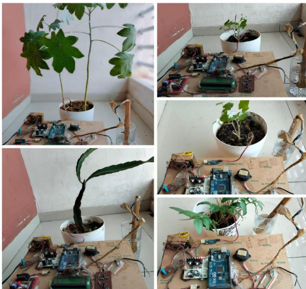
Figure 5: Experimental Setup of all five plants
